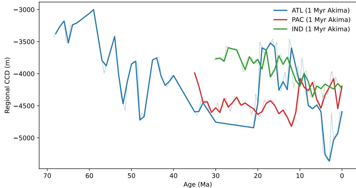
Regional CCD curves: raw 0.5 Myr (faint) and 1 Myr Akima resample
