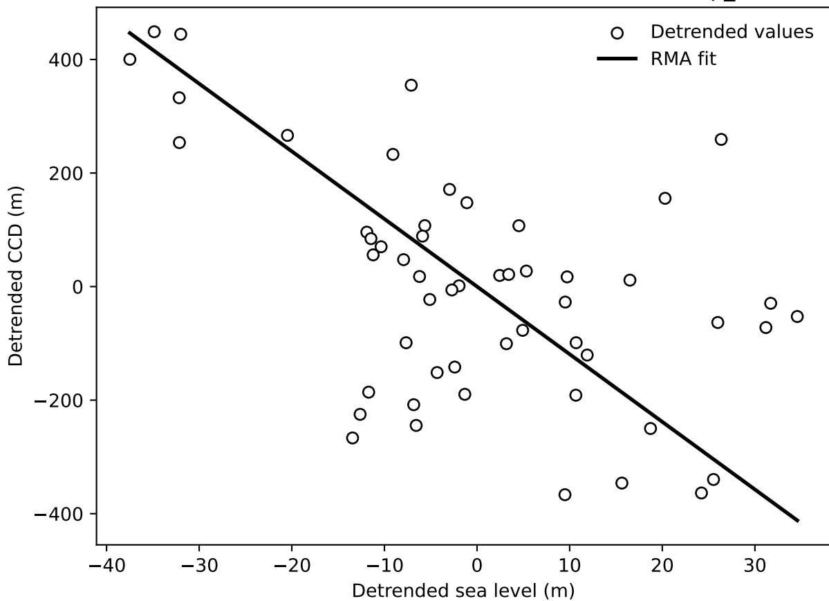
Detrended sea level vs CCD, 0-52 Ma ( r=-0.53 , R^2=0.28 , p\_AR1=0.24 )
