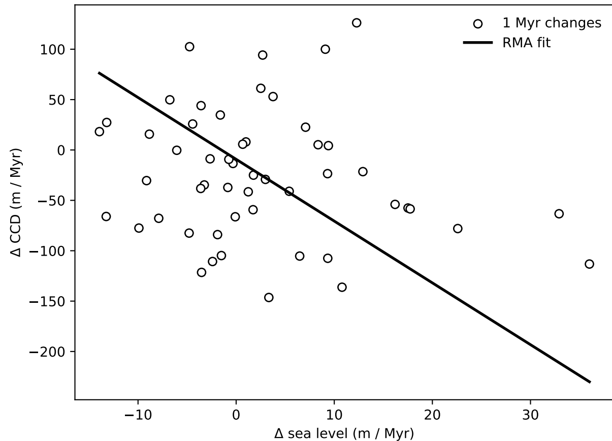
First-difference sea level vs CCD, 0-52 Ma ( r=-0.19 , R^2=0.04 )
