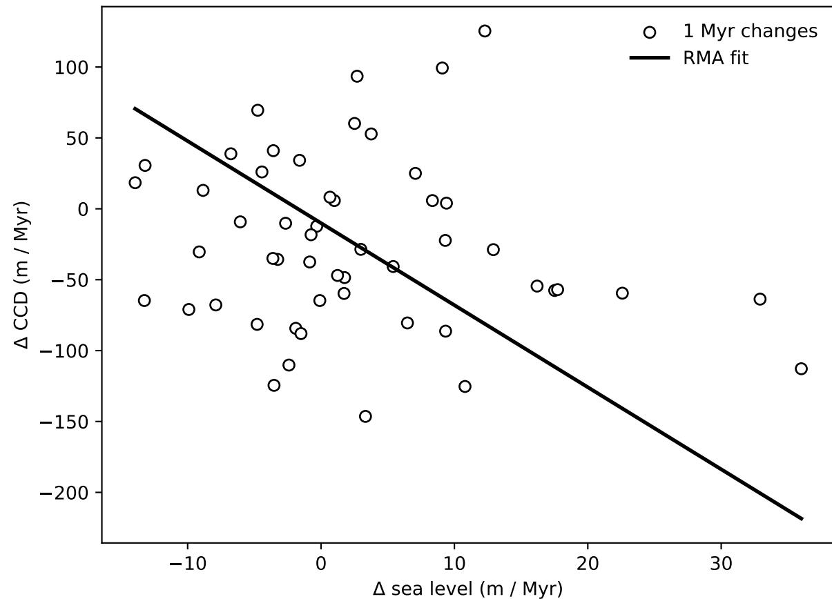
First-difference sea level vs CCD, 0-52 Ma ( r=-0.17 , R^2=0.03 )
