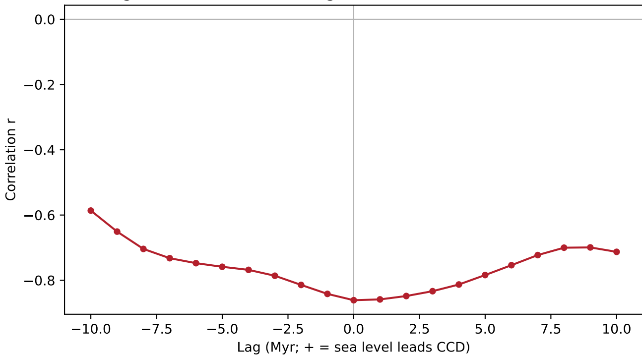
Lag correlation between long-term sea level and CCD, 0-52 Ma
