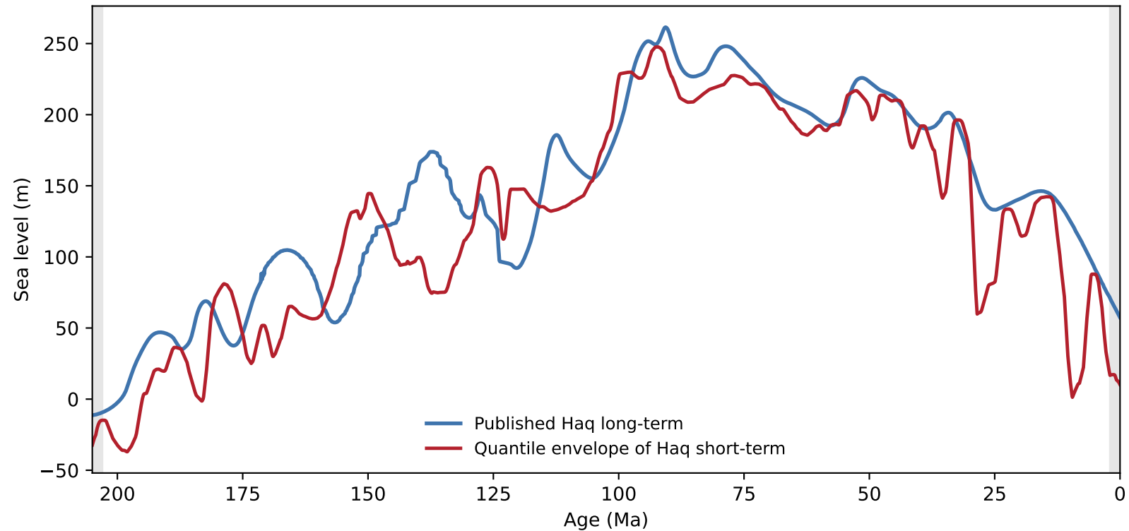
Validation of the peak-following operator ( r=0.90 , RMSE=36.4 m, MAE=27.6 m)
