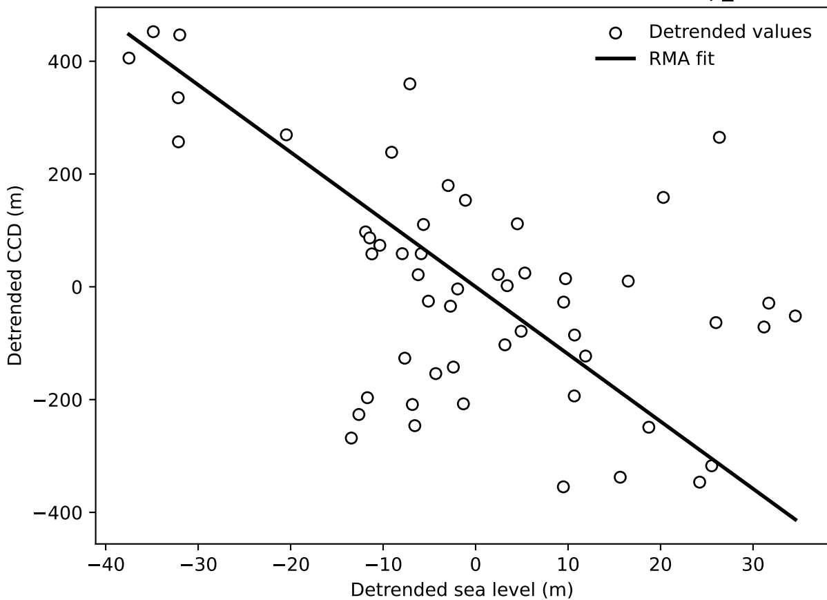
Detrended sea level vs CCD, 0-52 Ma ( r=-0.52 , R^2=0.28 , p\_AR1=0.26 )
