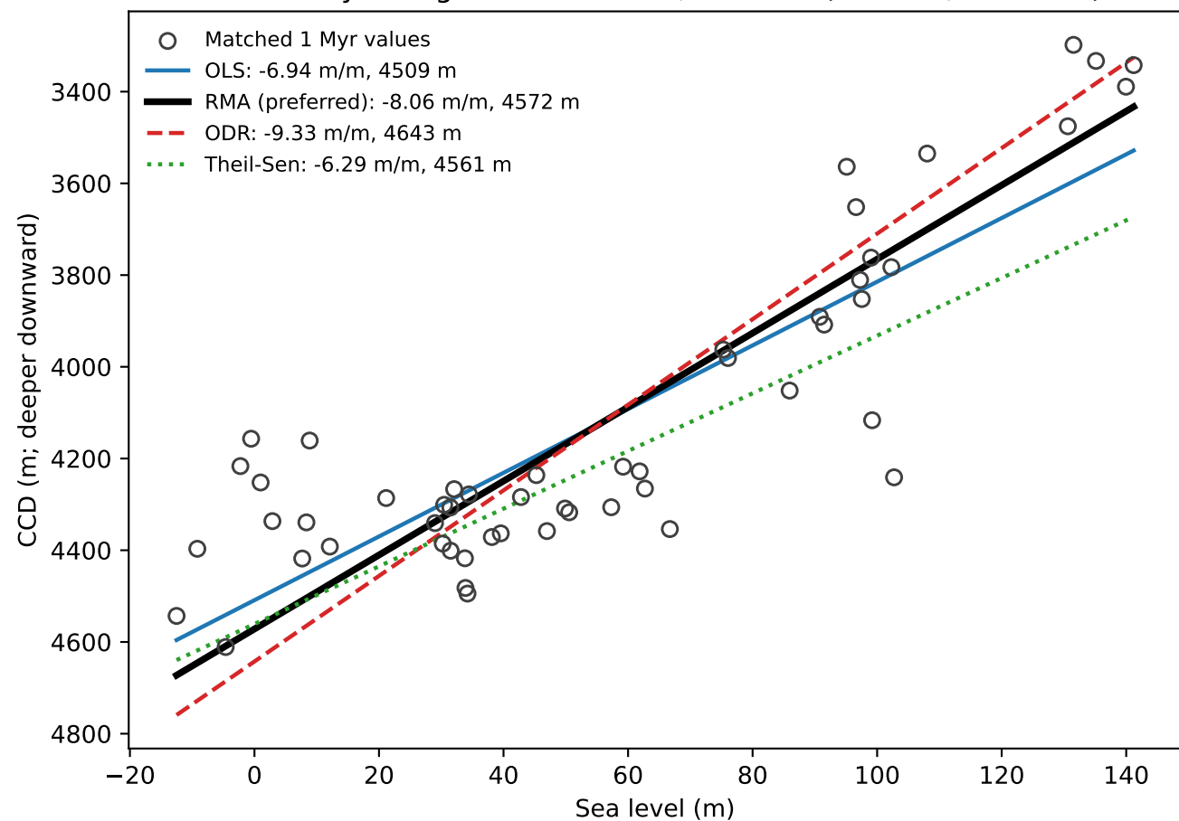
Sensitivity to regression method, 0-52 Ma ( r=-0.86 , R^2=0.74 )
