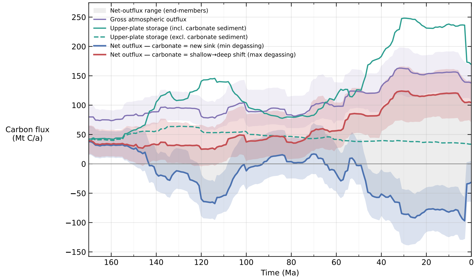
Net atmospheric carbon outflux — end-member carbonate scenarios — DM2026
