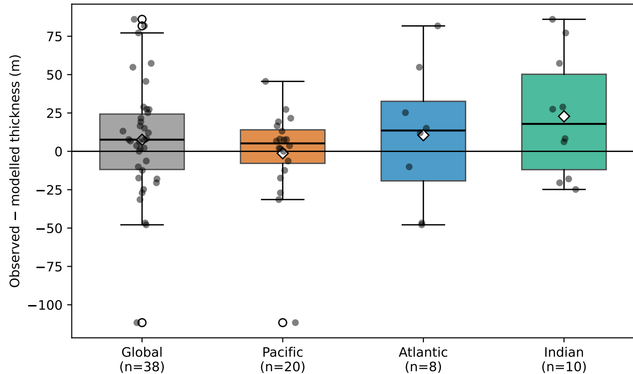
Difference by ocean basin (central / mean grid)
