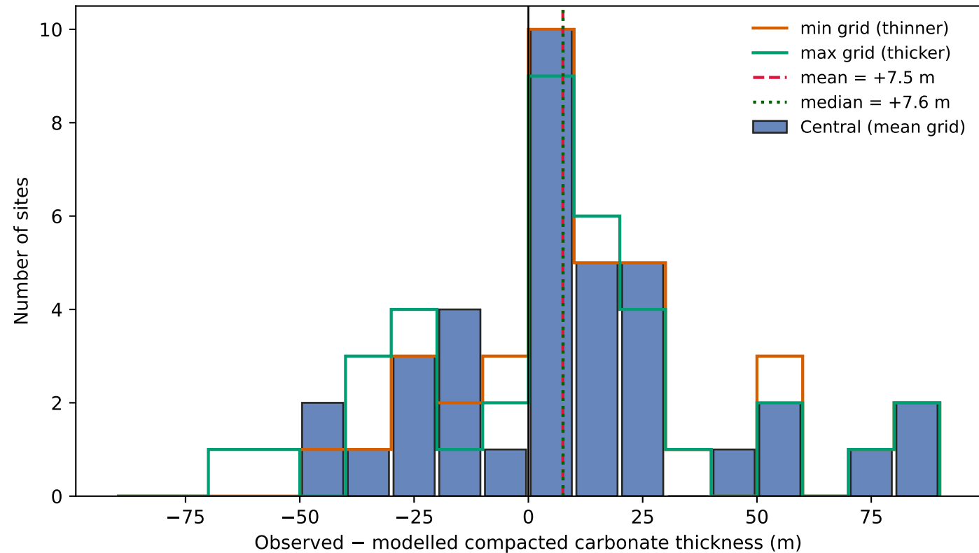
Difference histogram with min/max uncertainty (n=38, RMS=37.7 m)
