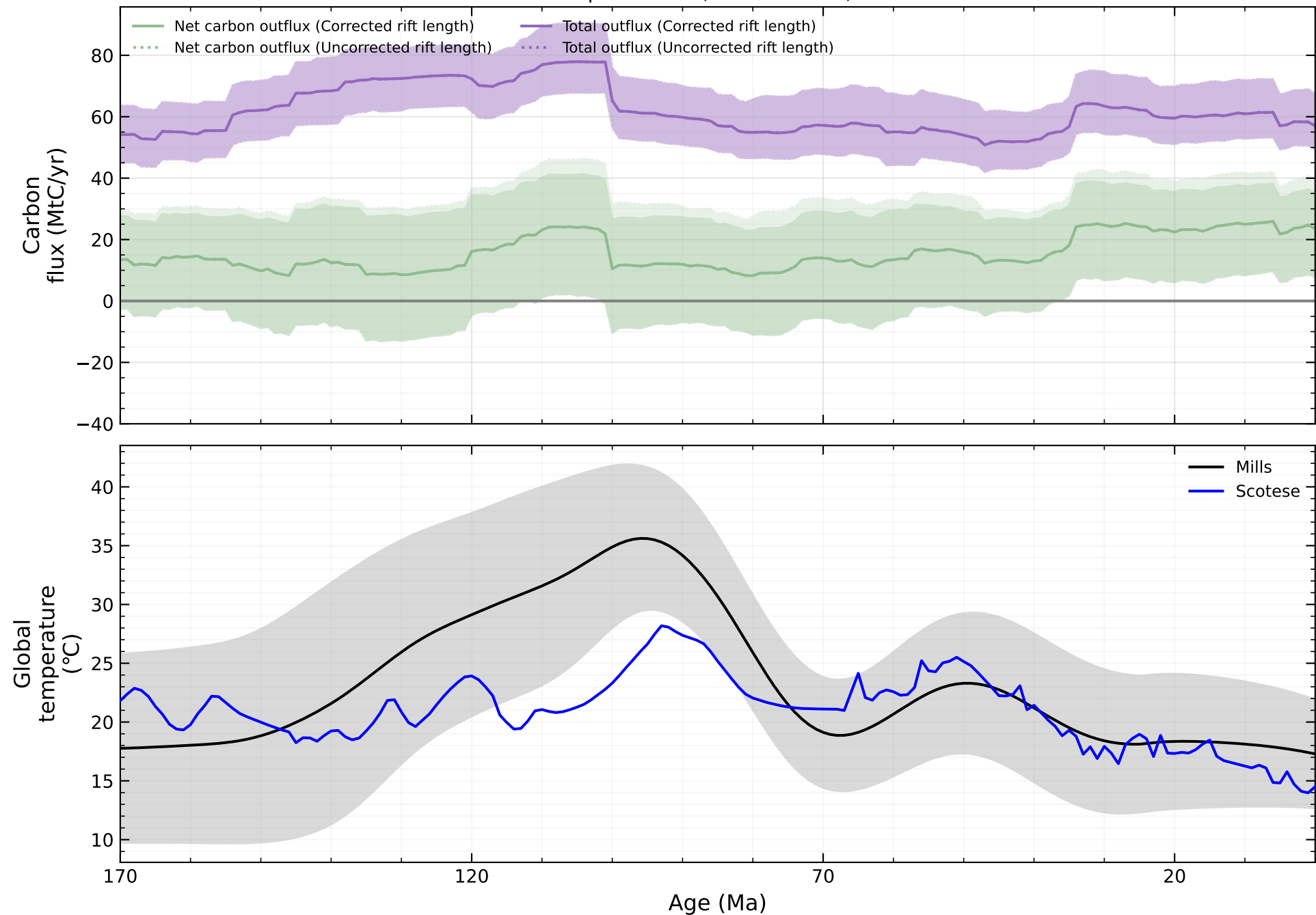
170 -> 0 Ma: net & total atmospheric flux (Ratschbacher) + GAST — DM2026
