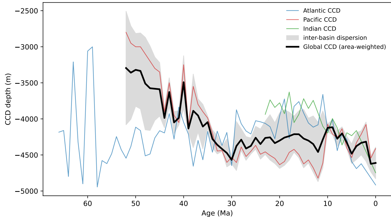
Global CCD synthesis with inter-basin dispersion, 0–52 Ma
