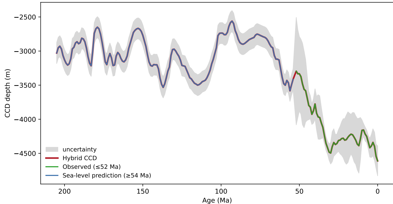
Hybrid CCD reconstruction with uncertainty, 0–205 Ma
