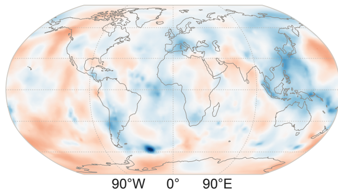
d GLAD-M35, P-wave
