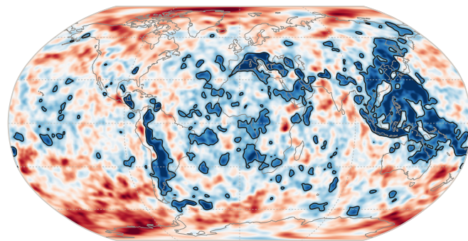
d GLAD-M35, P-wave
