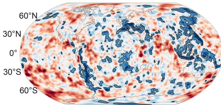
c GLAD-M35, S-wave
