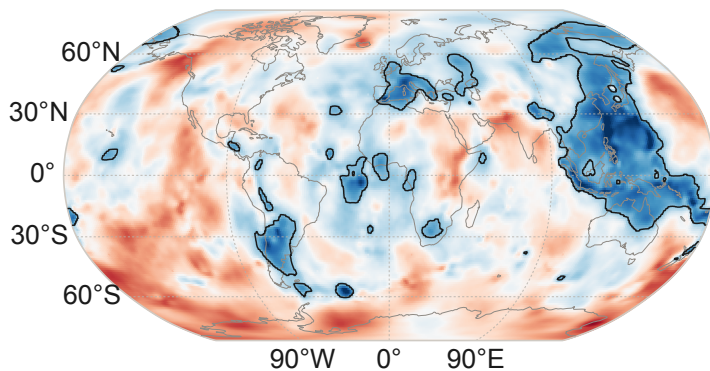
c GLAD-M35, S-wave
