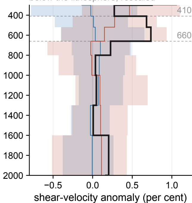
below the lithosphere, rescaled
