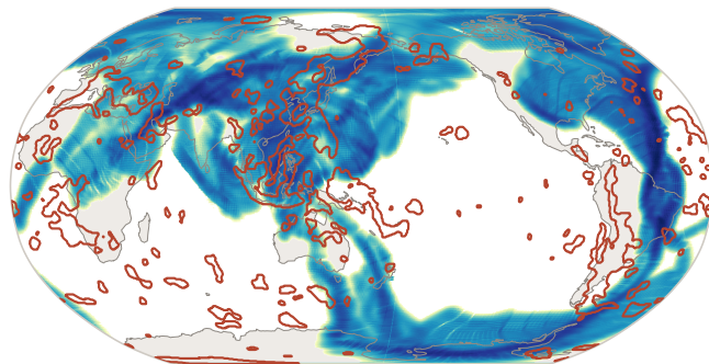
d 200–400 Ma
