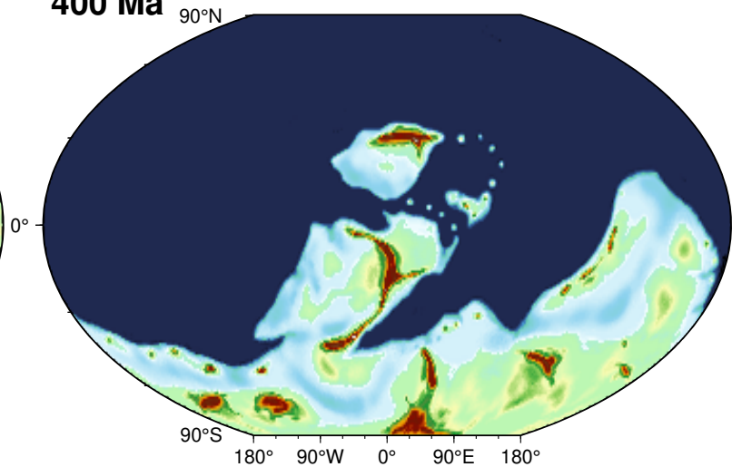
400 Ma Corrected
