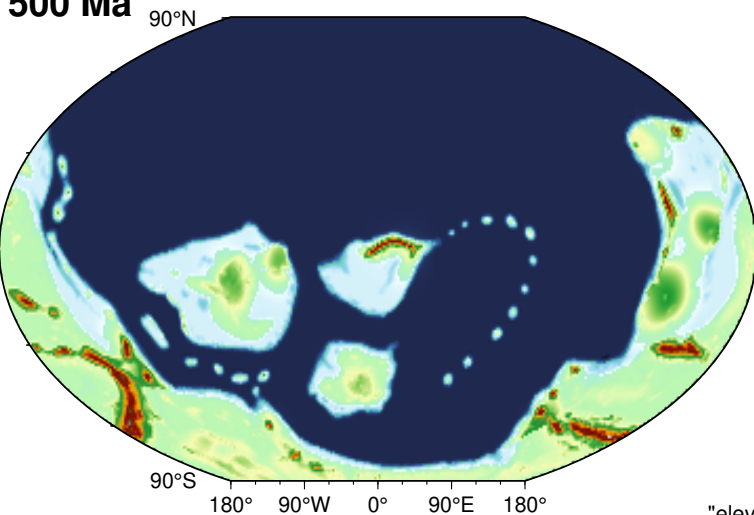
500 Ma Corrected
