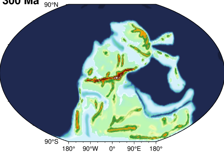
300 Ma Corrected
