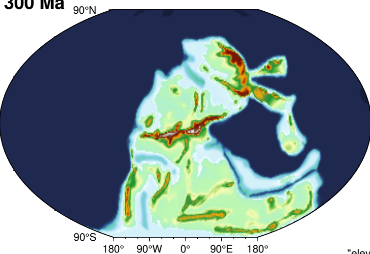
300 Ma Corrected
