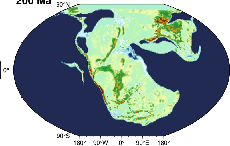
200 Ma Corrected
