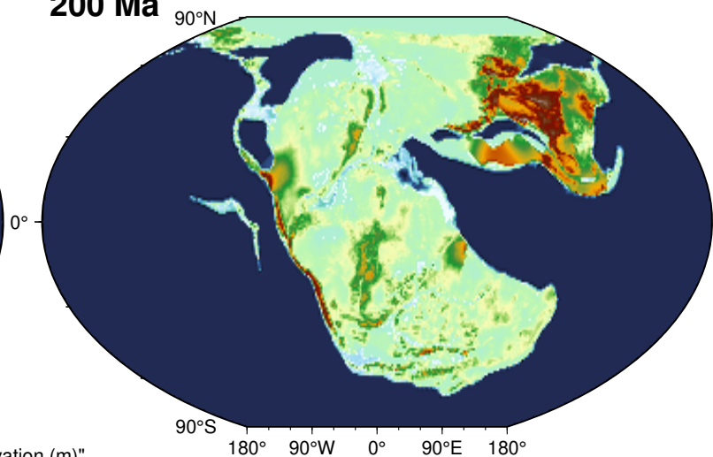
200 Ma Corrected
