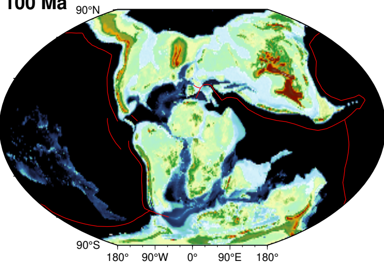
100 Ma Corrected
