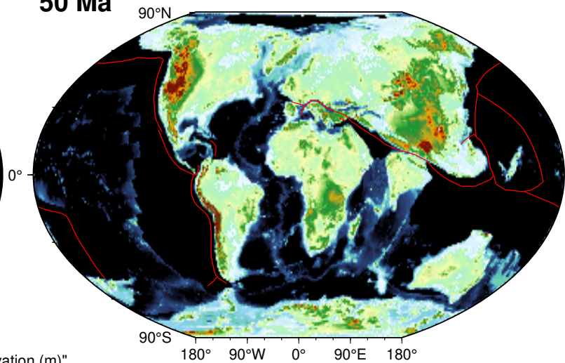
50 Ma Corrected
