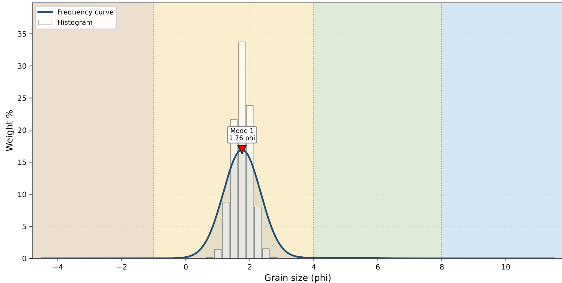
BCH-01 - Frequency distribution curve (unimodal)
