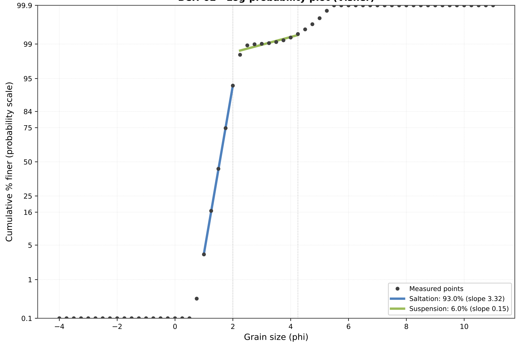
BCH-02 - Log-probability plot (Visher)
