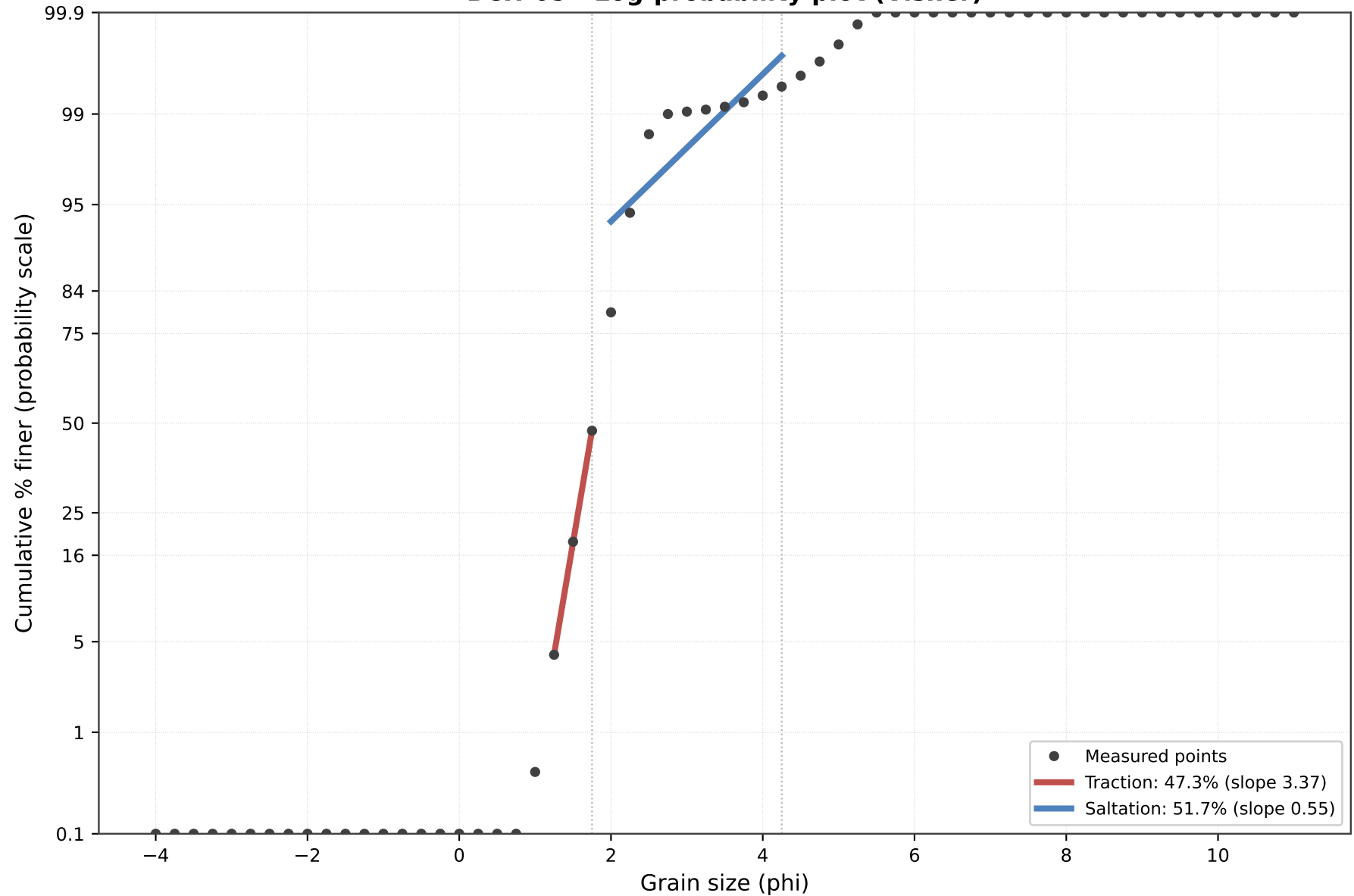
BCH-05 - Log-probability plot (Visher)
