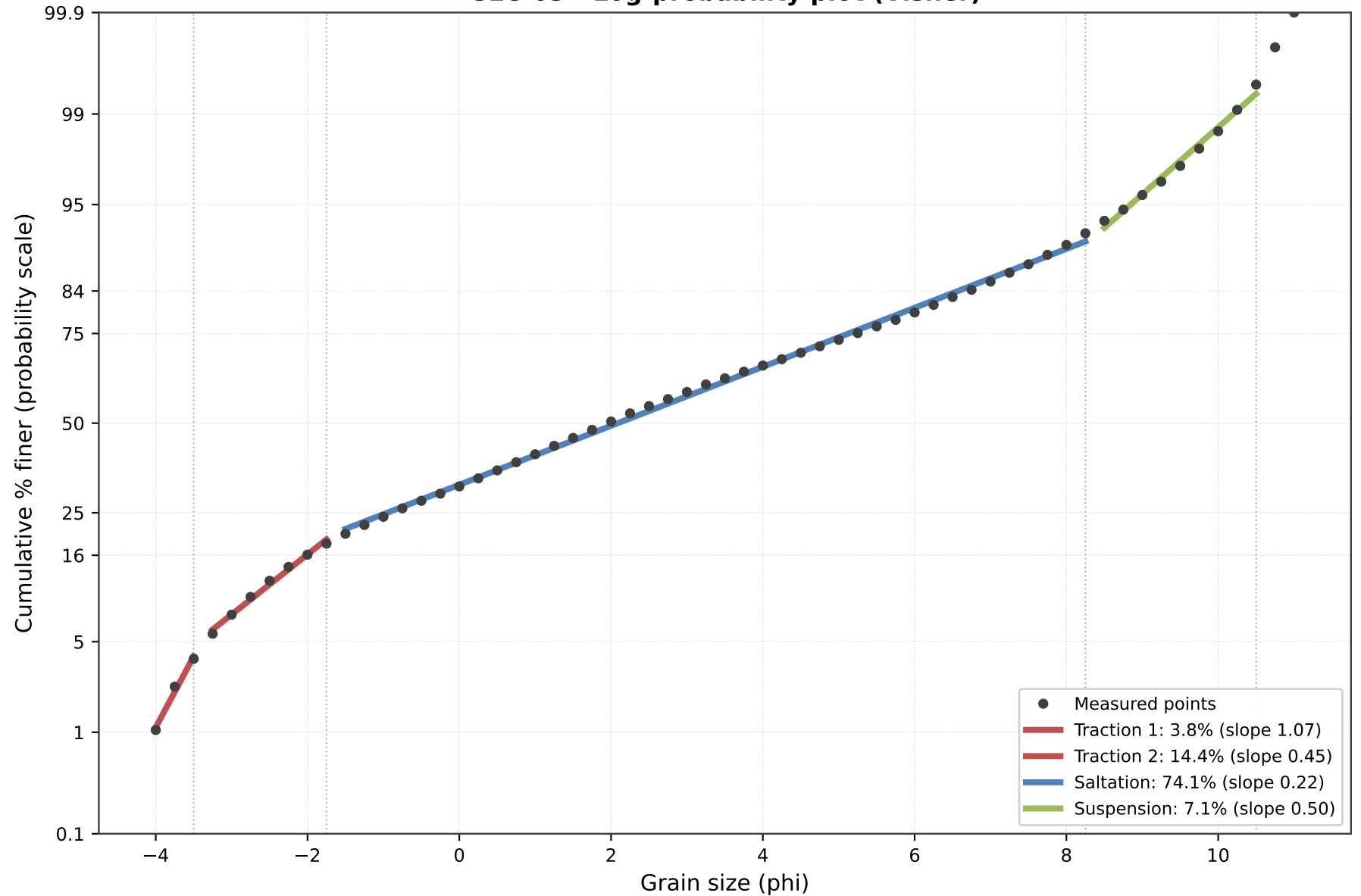
GLC-03 - Log-probability plot (Visher)
