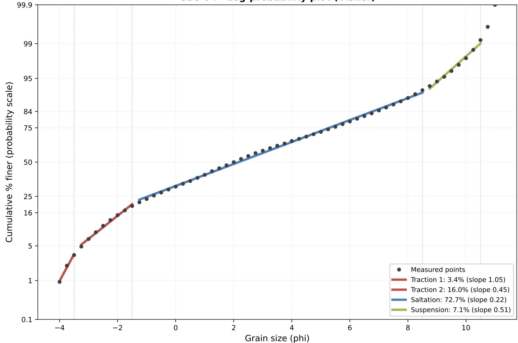
GLC-04 - Log-probability plot (Visher)
