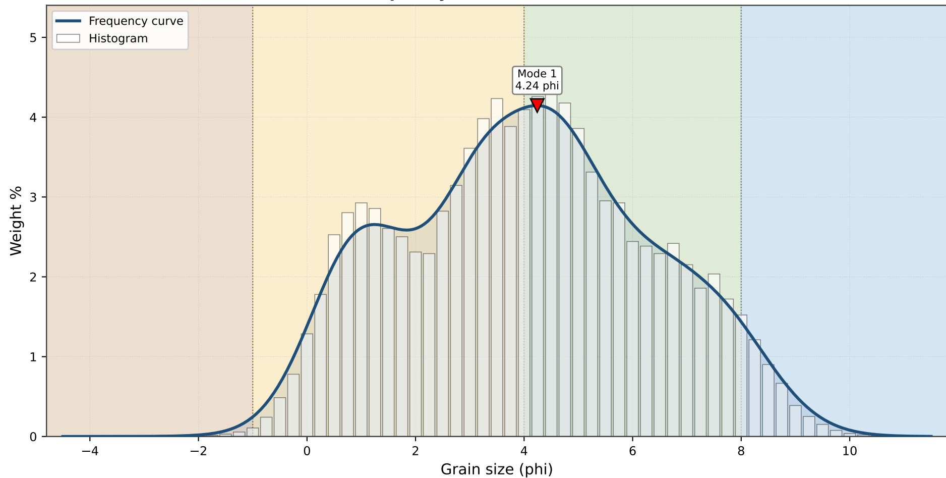
TRB-01 - Frequency distribution curve (unimodal)
