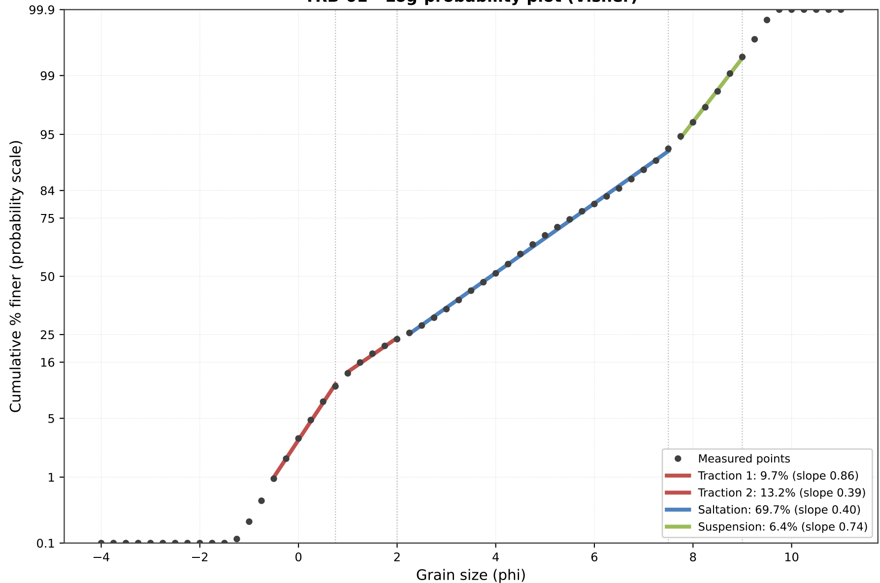
TRB-01 - Log-probability plot (Visher)
