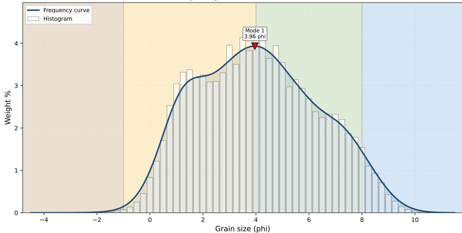
TRB-04 - Frequency distribution curve (unimodal)
