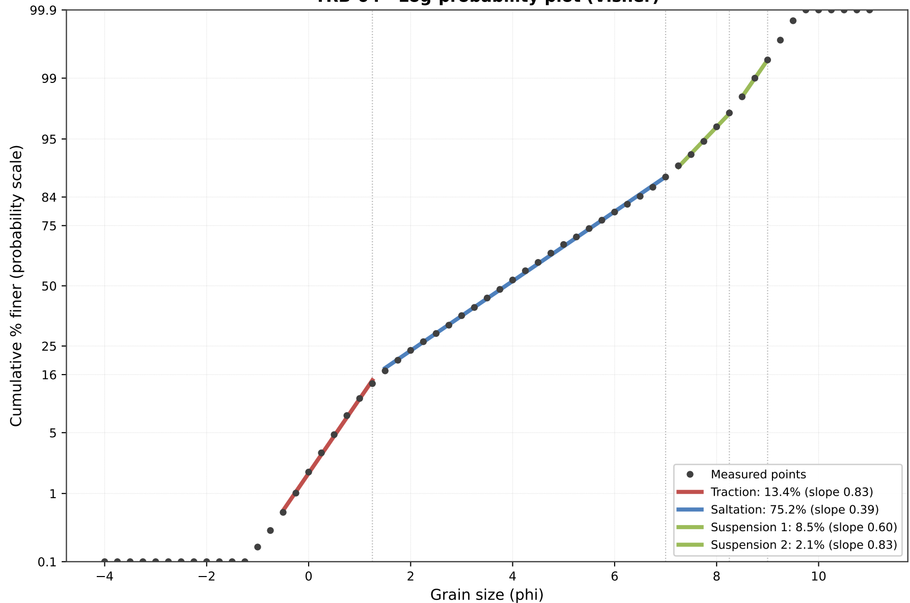
TRB-04 - Log-probability plot (Visher)
