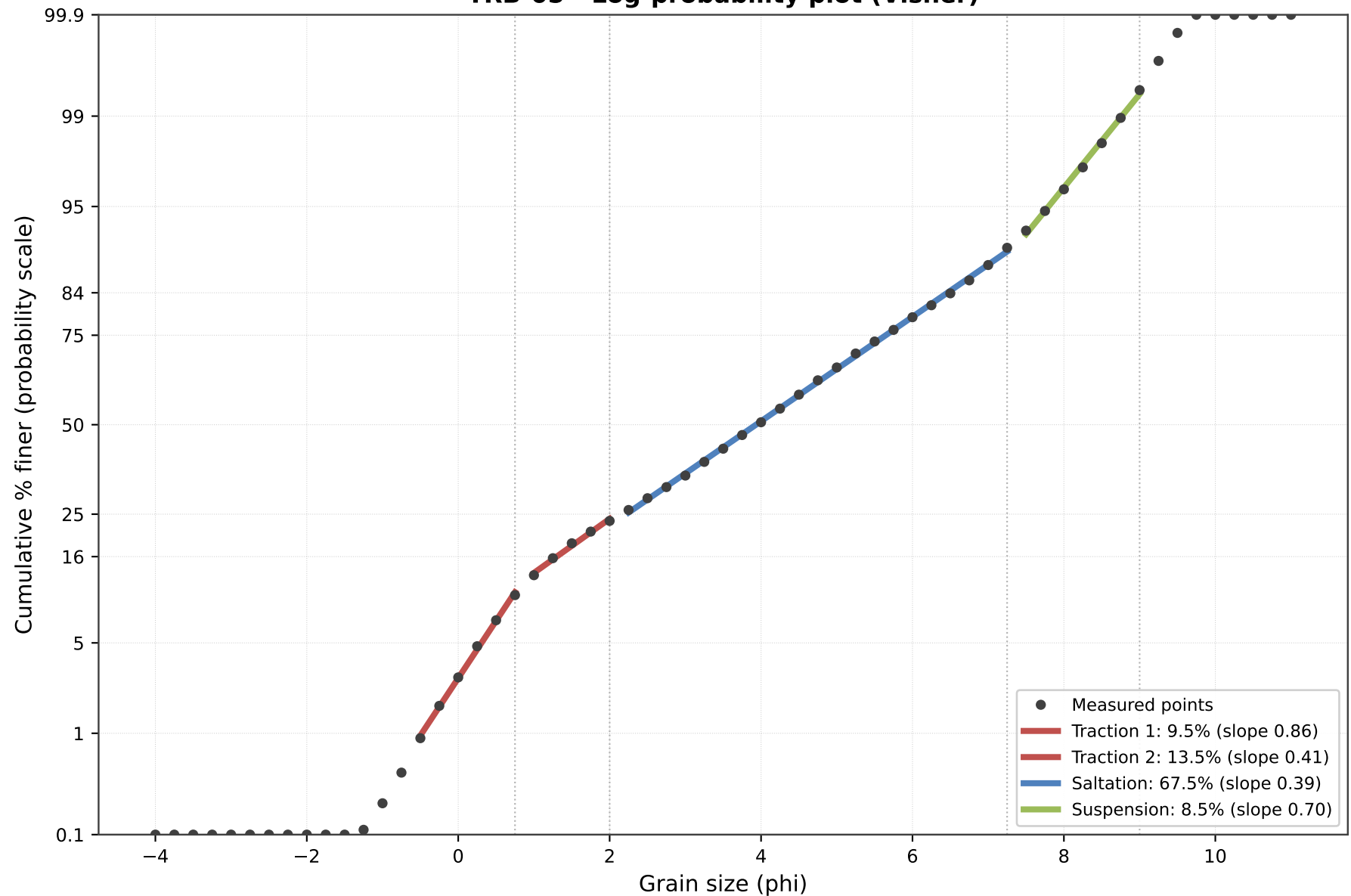
TRB-05 - Log-probability plot (Visher)
