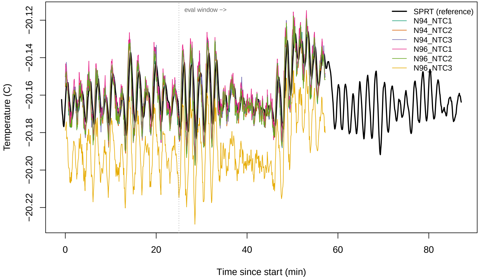
ntc2test: absolute temperature course (SPRT + NTCs)
