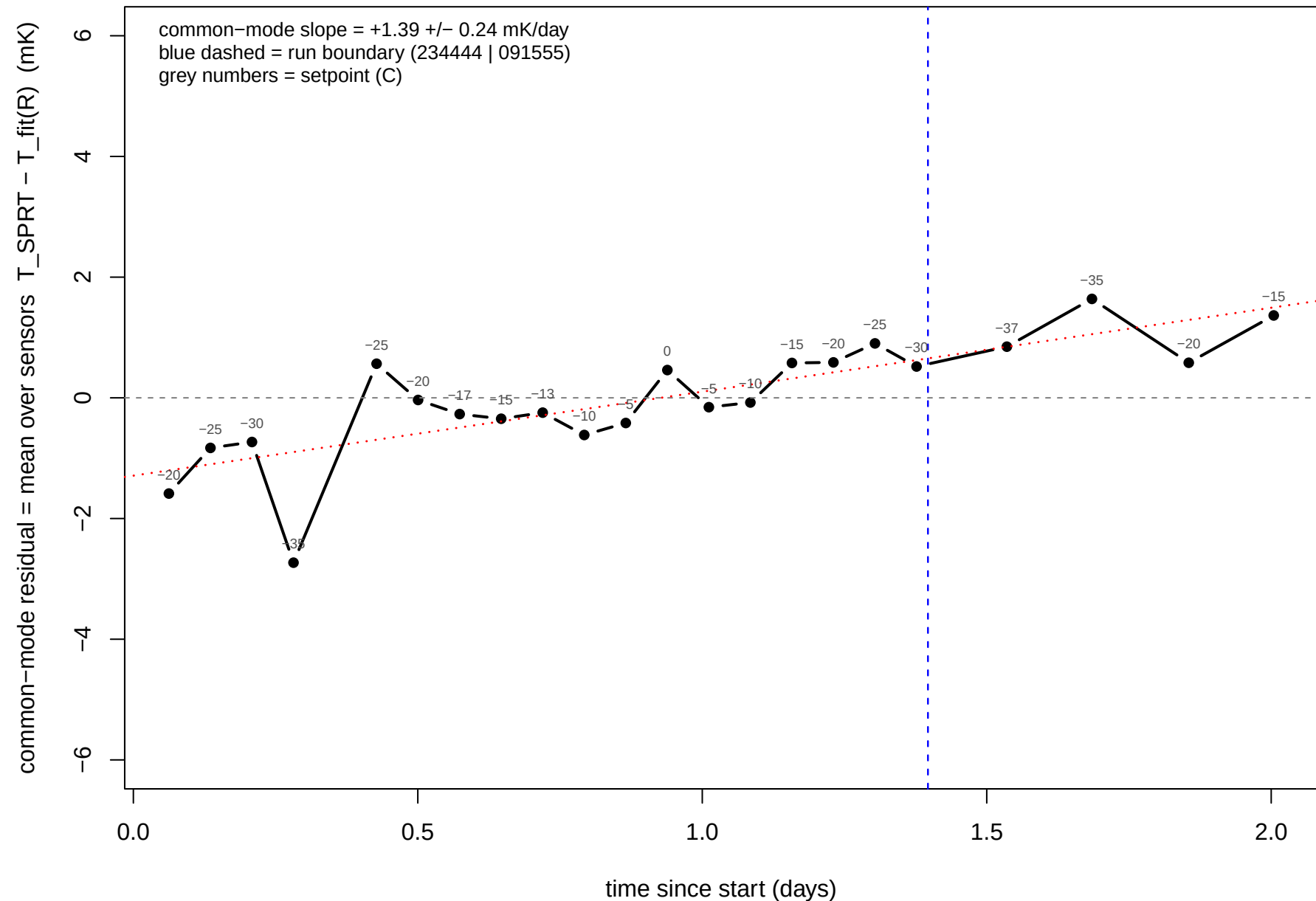
Common-mode residual vs time (shared by all sensors: reference / bath)
