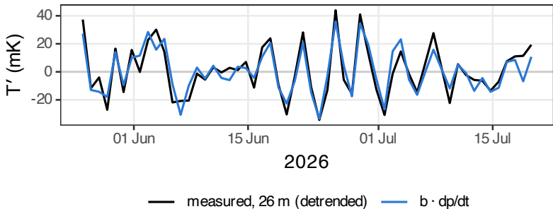
Temperature in the open hole, B40
