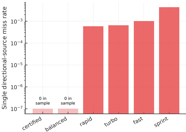
Discovery risk
