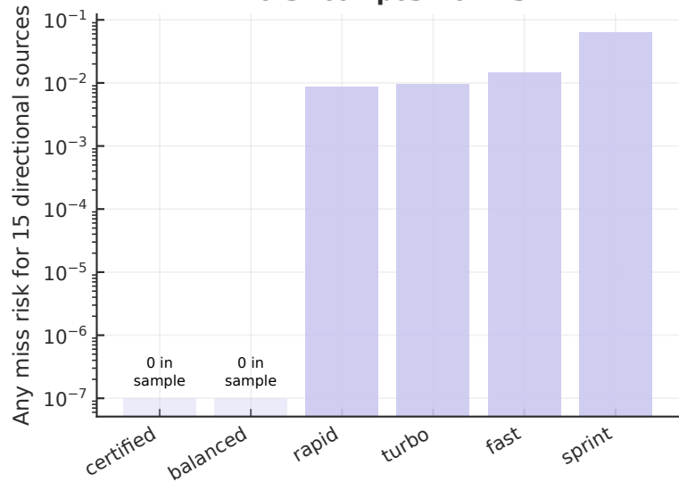
Worst-composition risk
