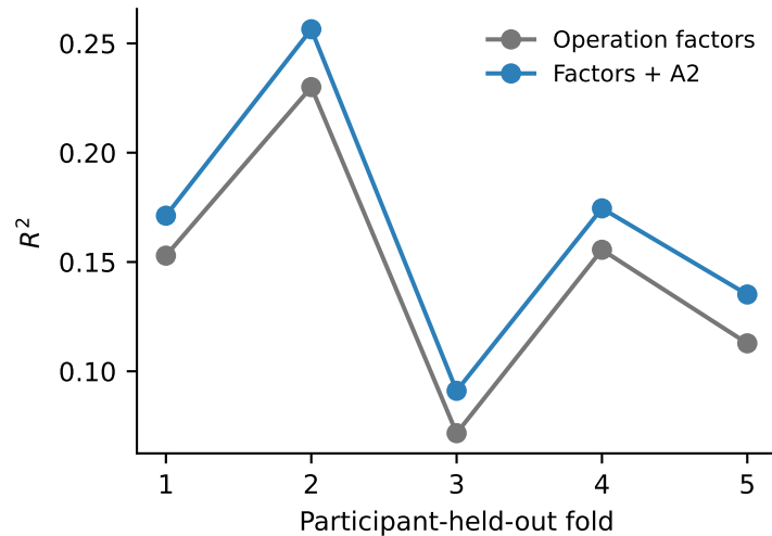
A. Held-out explained variance
