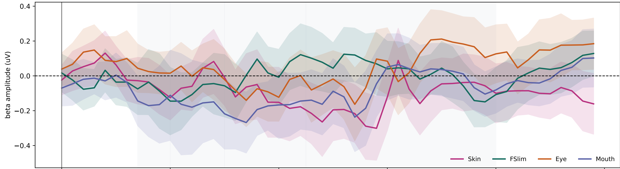
Trial-level GLM beta time courses
