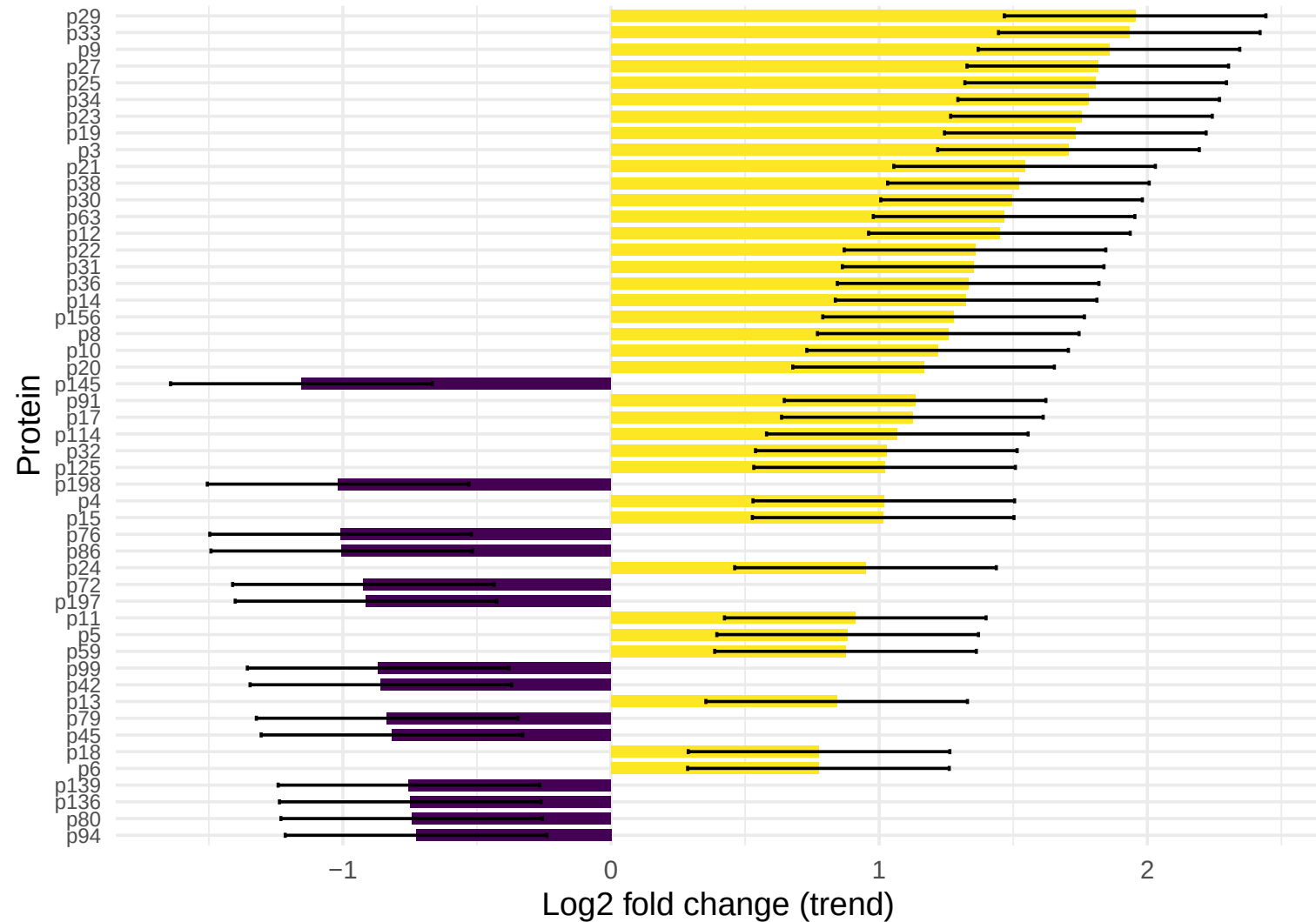
Top 50 proteins by |\log FC|
