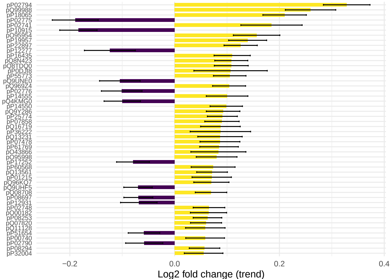
Top 50 proteins by |\log FC|
