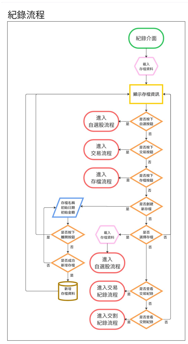
Figure 6: 紀錄選單流程圖
