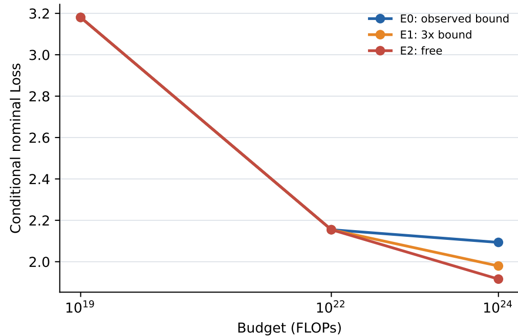
Evidence boundary changes high-budget conclusions
