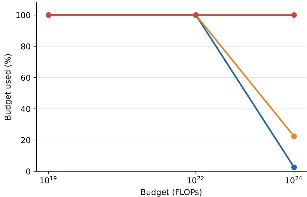
Evidence boundary changes high-budget conclusions
