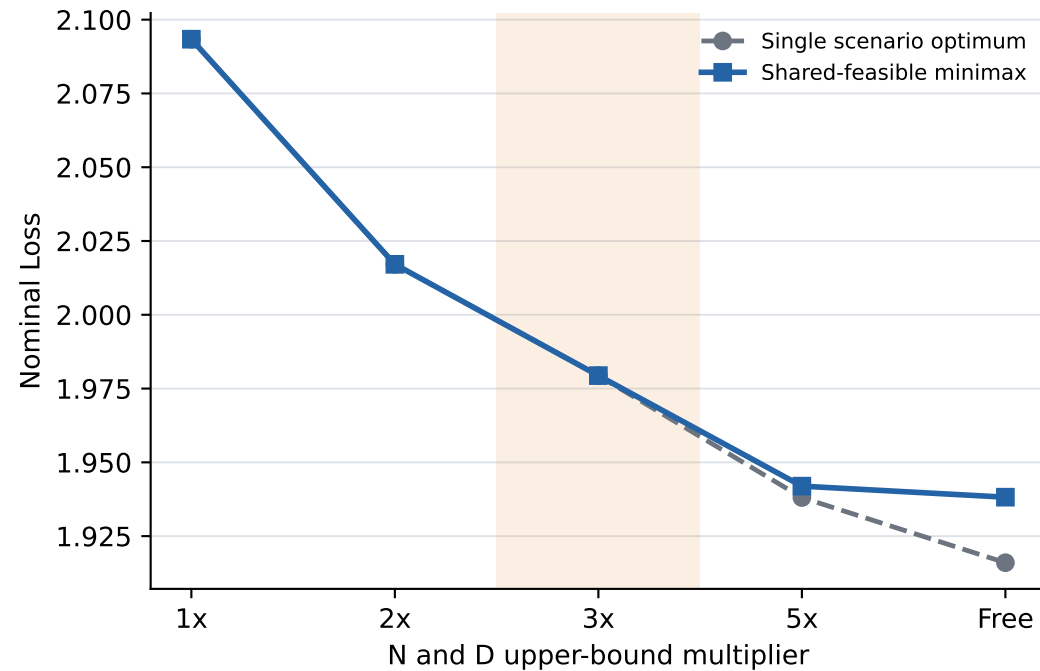
10^{24} FLOPs: loss and extrapolation-bound trade-off
