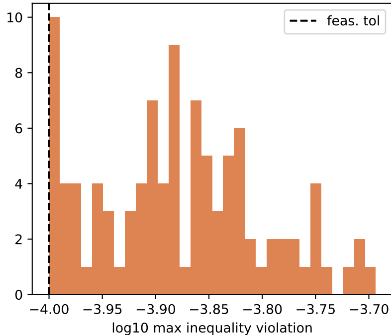
DC3 constraint violation
