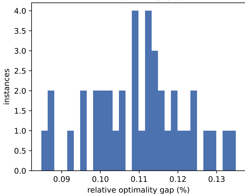
DC3 optimality gap
