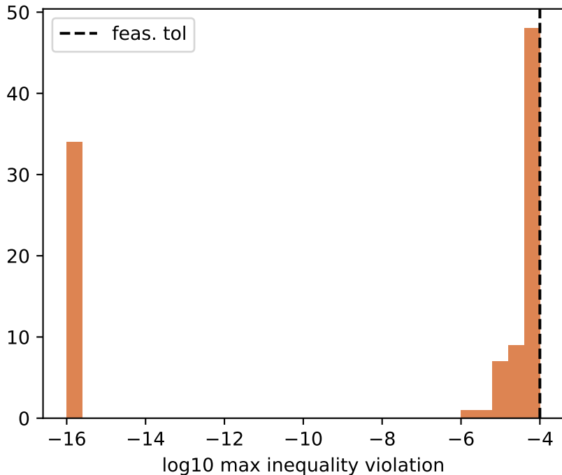
DC3 constraint violation
