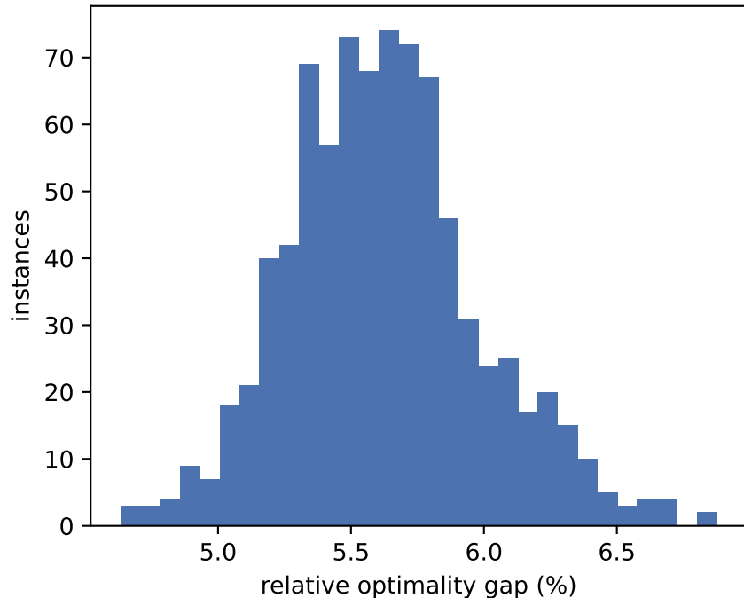
DC3 optimality gap
