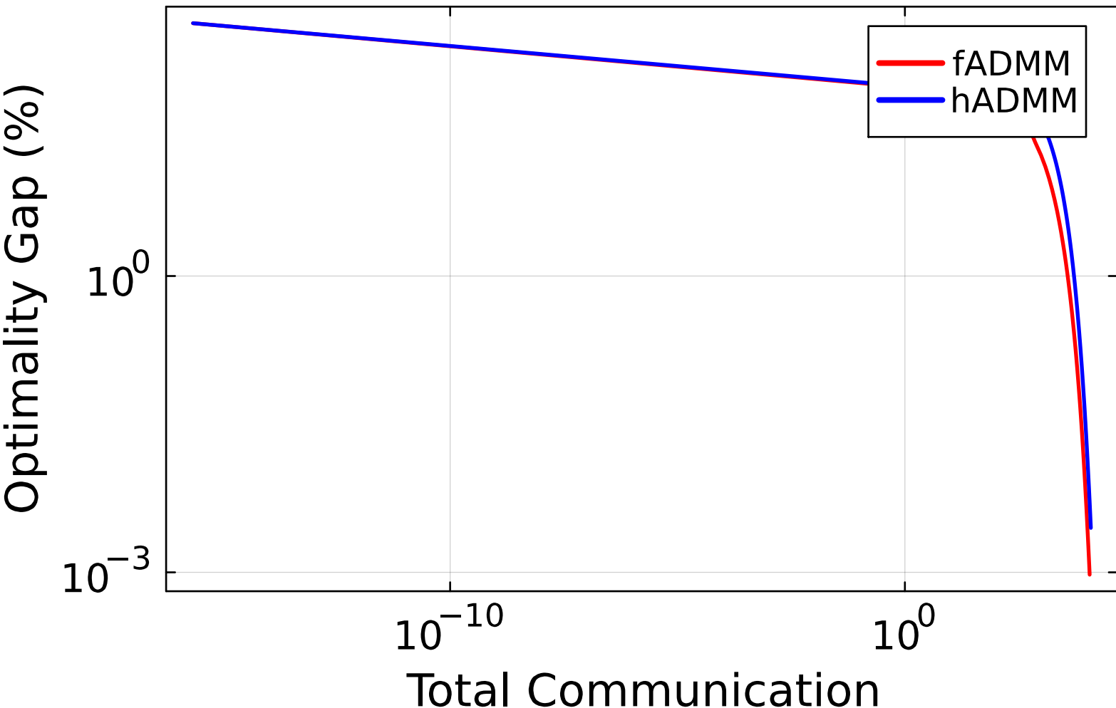
Worst Optimality Gap: Topology 6
