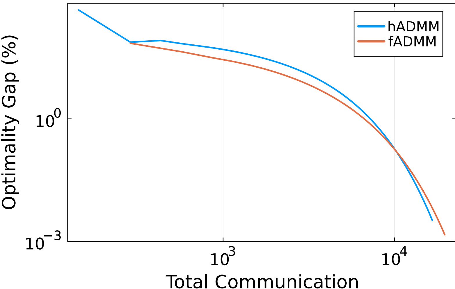
Max Communication: Topology 8
