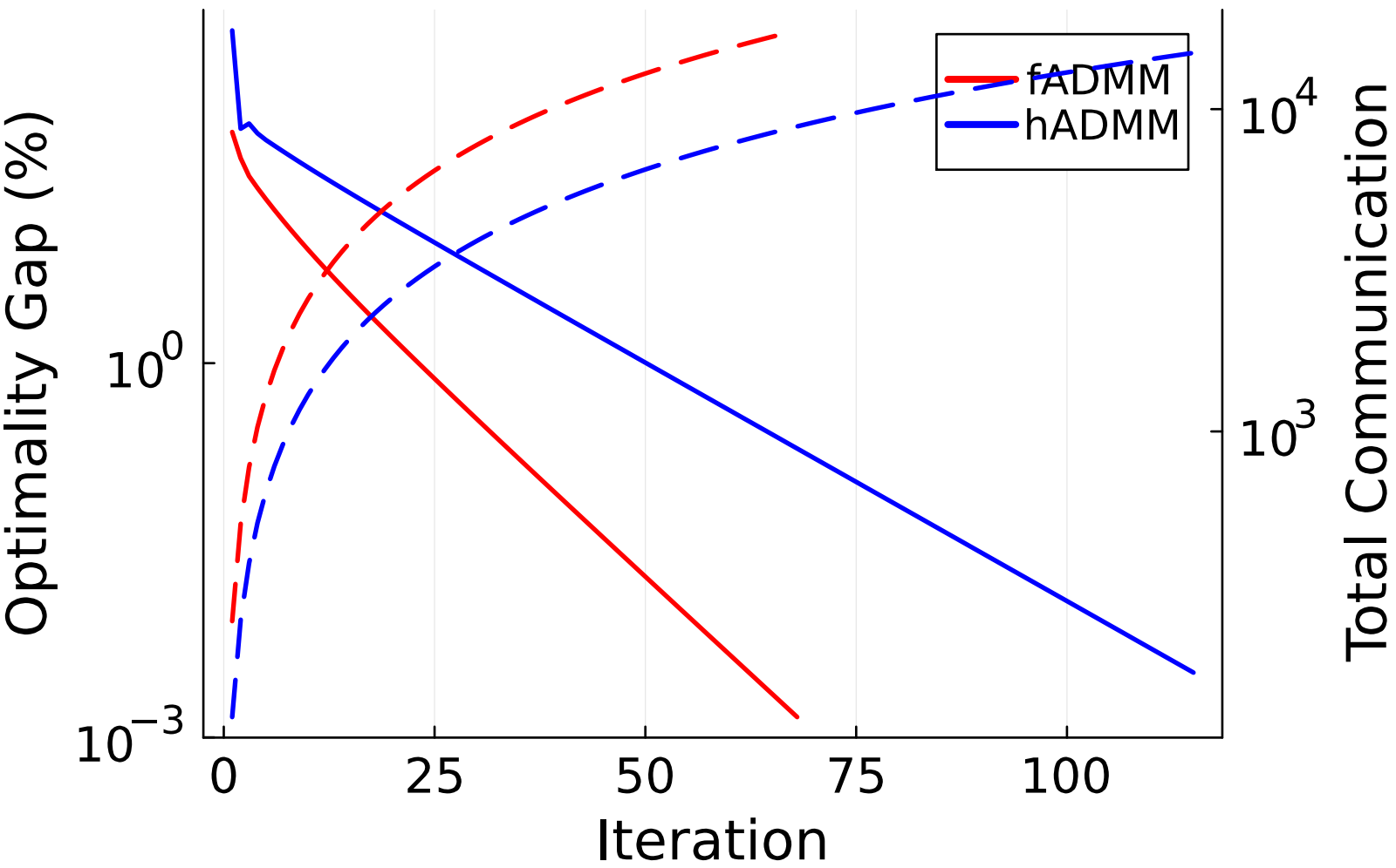
Worst Optimality Gap: Topology 24
