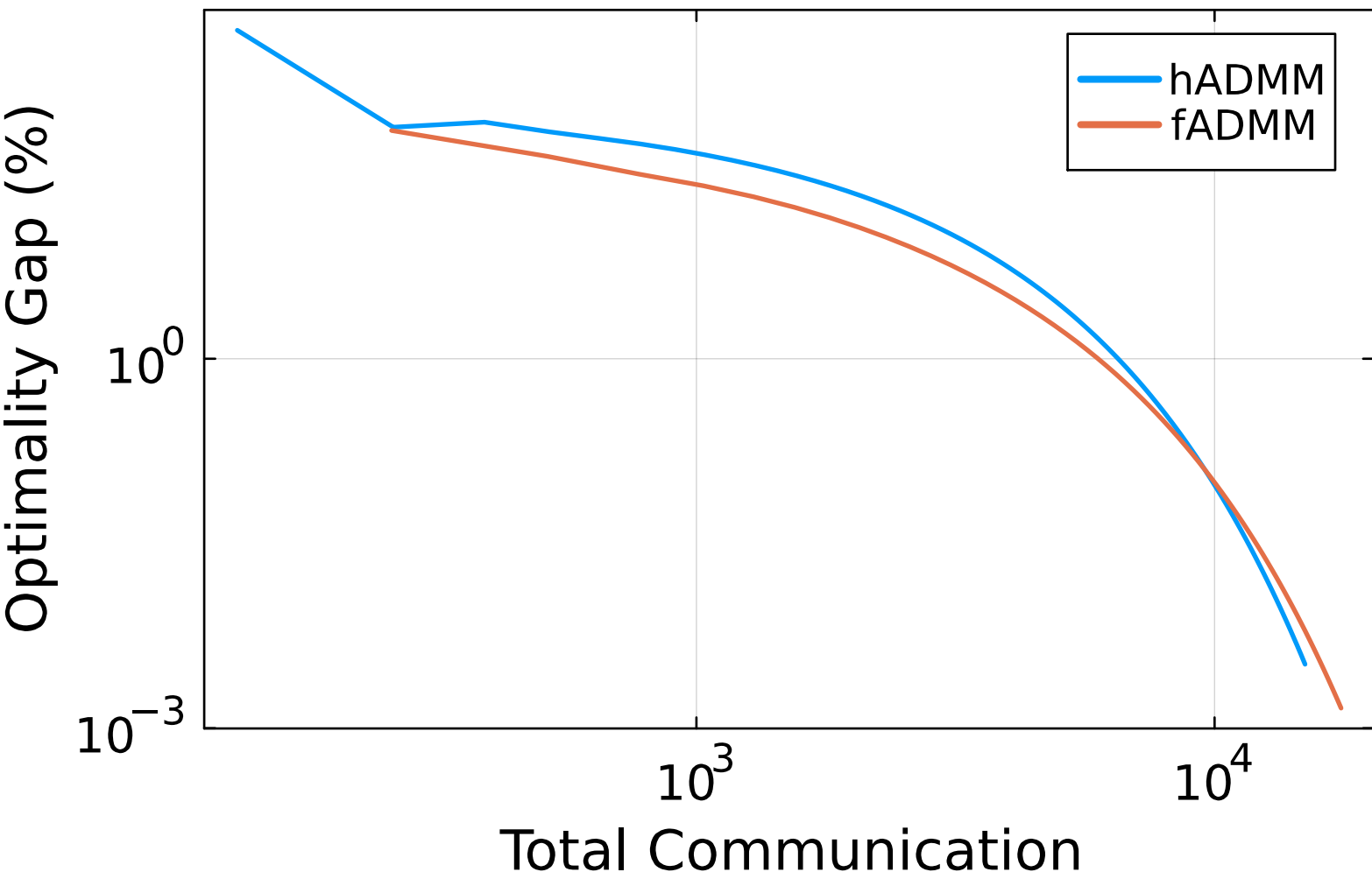
Worst Optimality Gap: Topology 24
