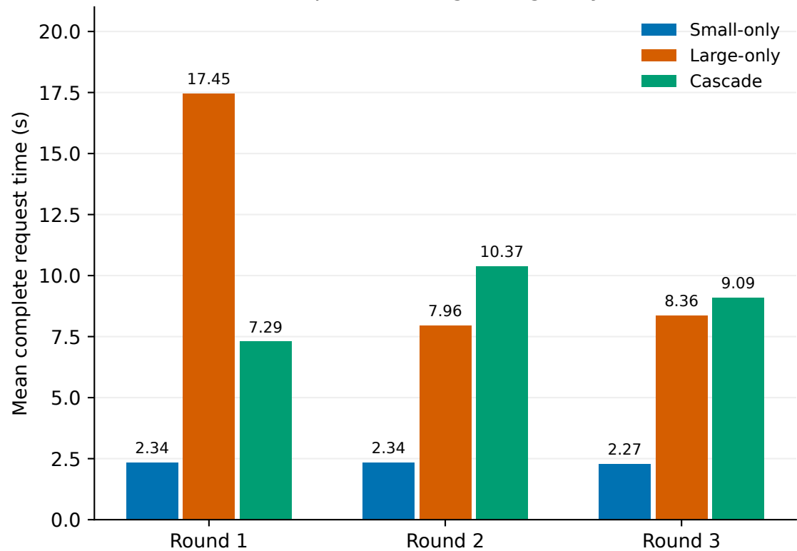
(b) The speed ranking changes by round
