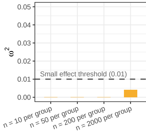
\omega^2 (effect size)
